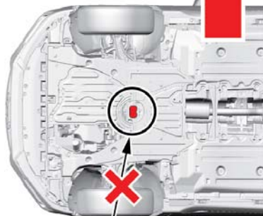
FRONT LIFT POINT
