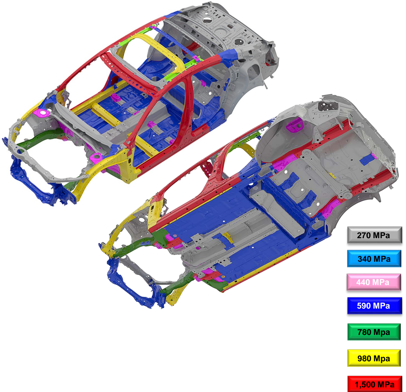
Steel Tensile Strength Legend
