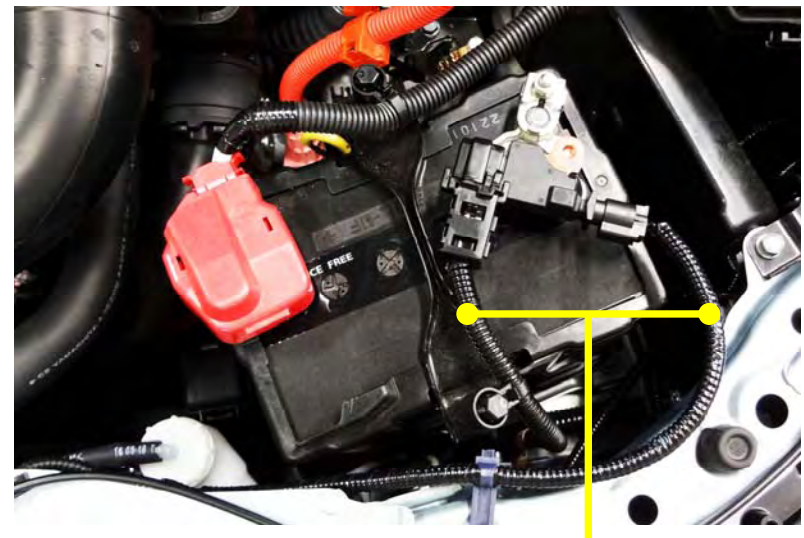
Negative Cables
